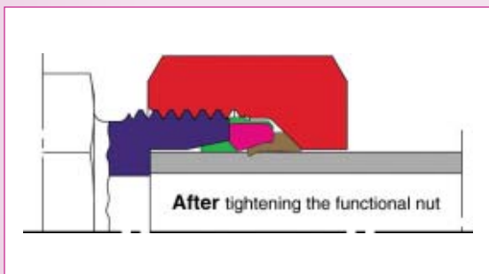
The metallic support of the sealing ring acts just like an integrated preassembly tool.
