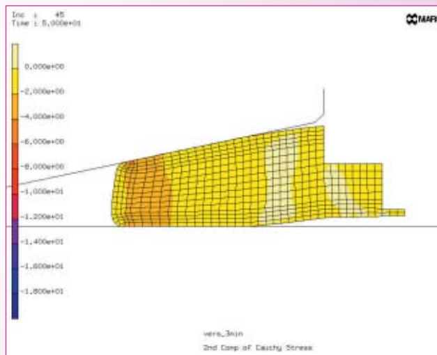
The metallic support of the sealing ring acts just like an integrated preassembly tool.
