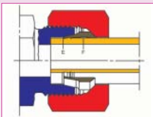
After tightening the nut
